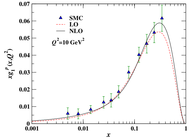
FIG. 9 (color online). Proton spin structure function at the LO and NLO approximations at Q^2 = 10 \text{ GeV}^2 and its comparison with SMC experimental data [22].
